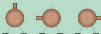
MMO Nozzle Orientation (viewed from bearing end)
