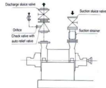
Fig.2-2 Check valve with auto relief valve
