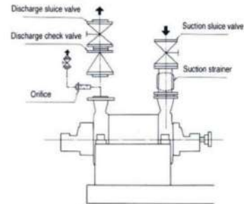
Fig.2-1 Relief valve
