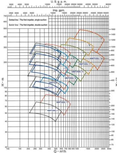
60Hz-4P (1750 1/min) — Mixed-flow Impeller
