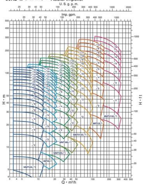
50Hz-4P (1450 1/min) — Radial Impeller
