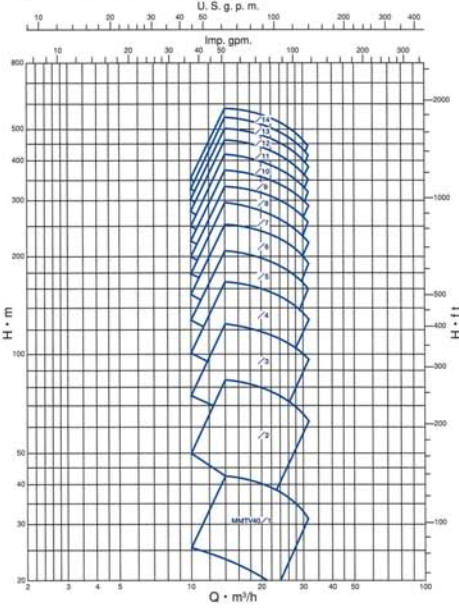
60Hz-2P (3500 1/min) — Radial Impeller
