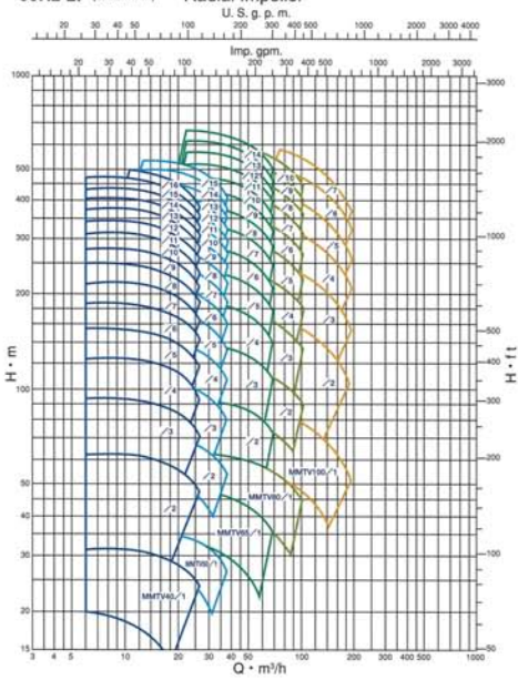
50Hz-2P (2900 1/min) — Radial Impeller
