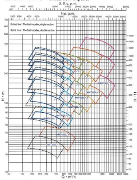
50Hz-4P (1450 1/min) — Mixed-flow Impeller
